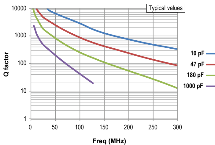
3838 - Q factor
