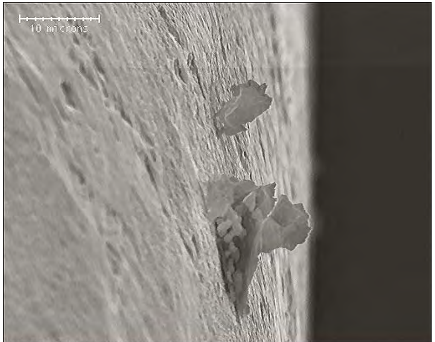
160S41W475KV4 #514-5389, 4000 hours
